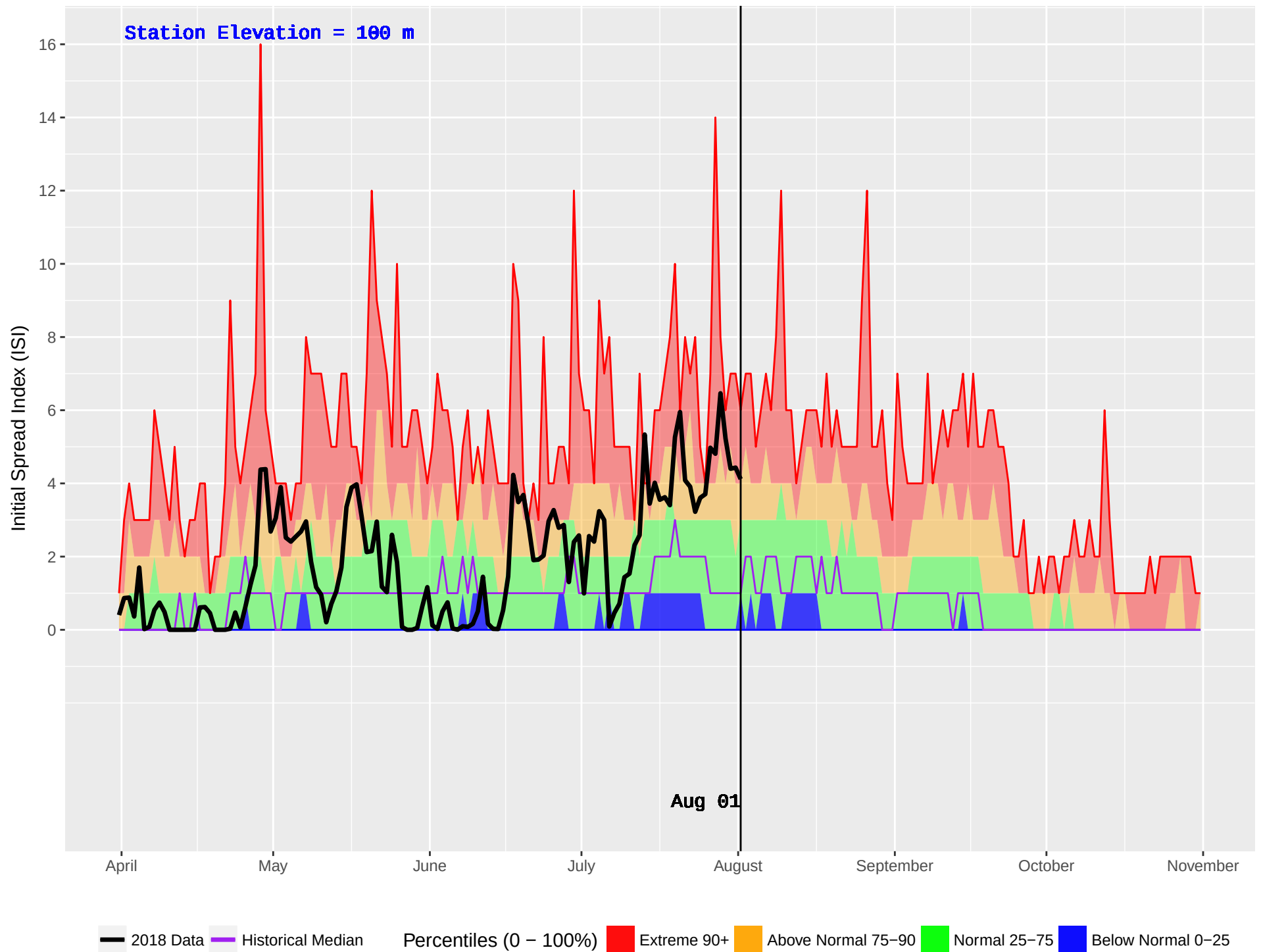
HONNA (93) : Historical (1986–2016) and Current (2018) Daily Initial Spread Index (ISI)
