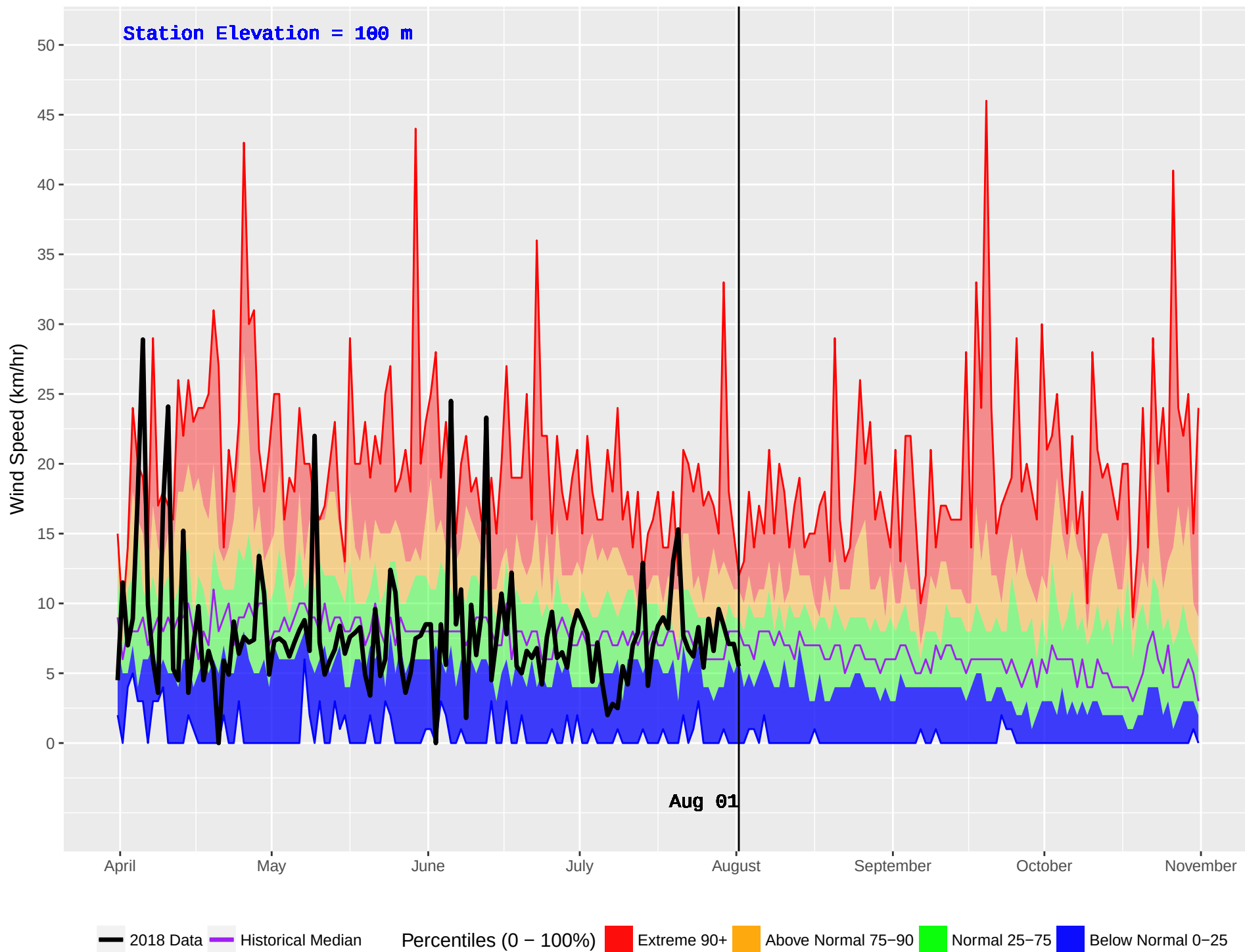
HONNA (93) : Historical (1986–2016) and Current (2018) Daily Wind Speed
