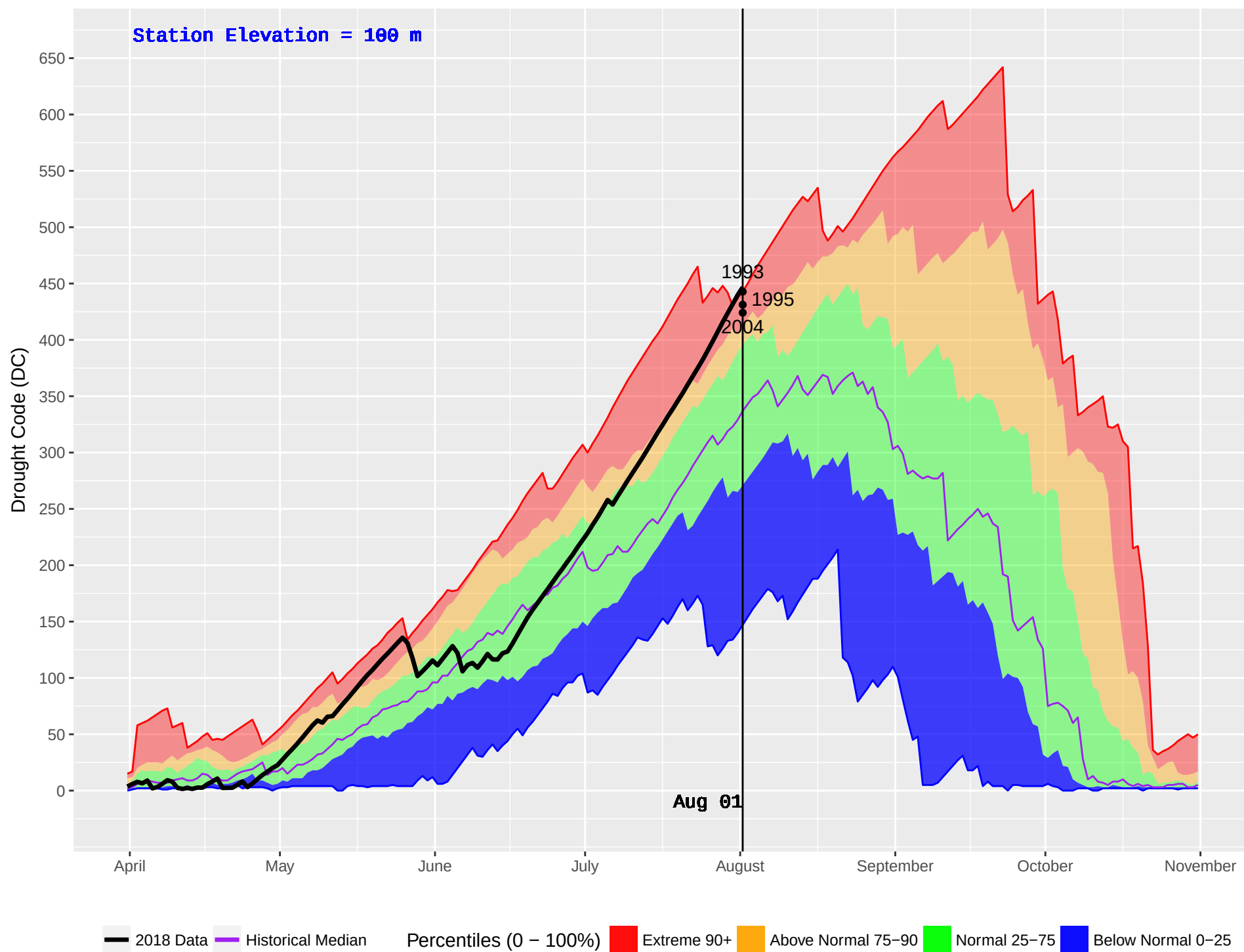
HONNA (93) : Historical (1986–2016) and Current (2018) Daily Drought Code (DC)
