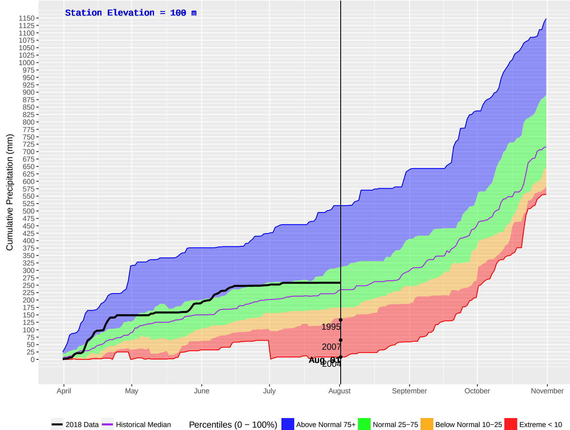
HONNA (93) : Historical (1986–2016) and Current (2018) Daily Cumulative Precipitation
