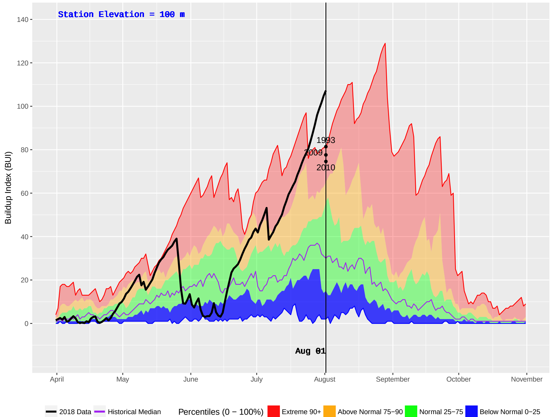
HONNA (93) : Historical (1986–2016) and Current (2018) Daily Buildup Index (BUI)
