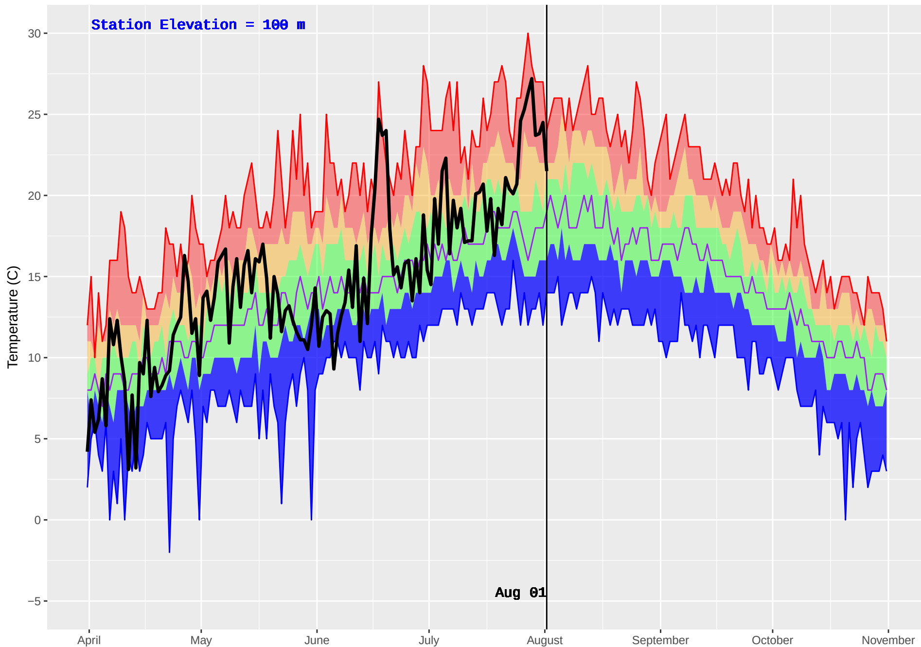
HONNA (93) : Historical (1986–2016) and Current (2018) Daily Temperature
